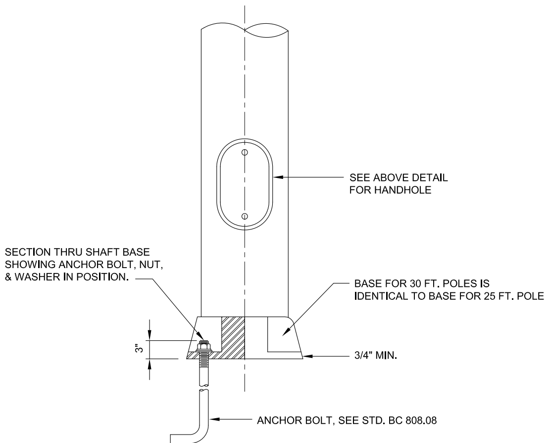
DETAILS OF ANCHOR BOLT IN PLACE
