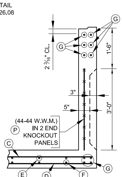
SECTION 2-2
