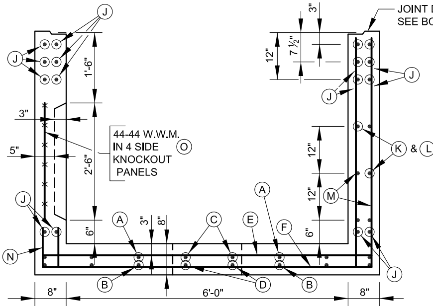
SECTION 1-1
